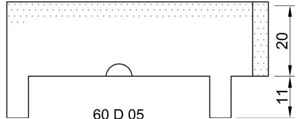
60 D 05 TAPA (PLS) (10 adet/paket)
