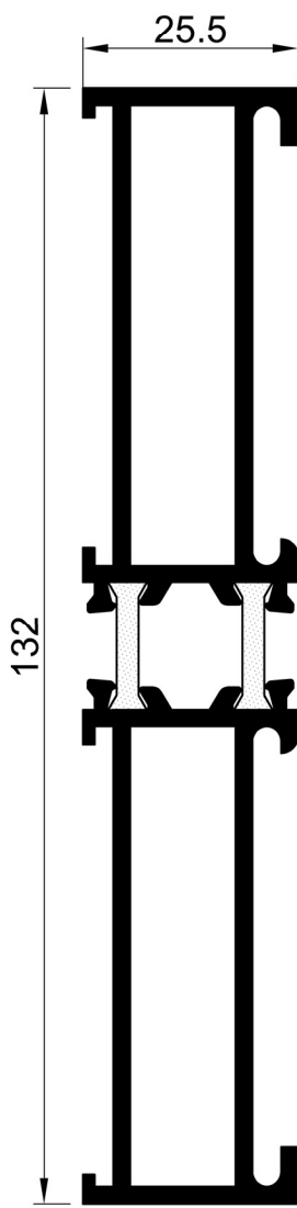
60 E 34 AĞIRLIK : 1.921 kg/m. JX: 123.69 cm 4 JY: 4.42 cm 4
