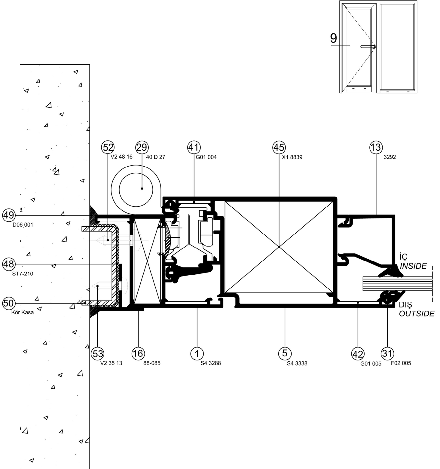
DETAIL ⑨ DETAYI
