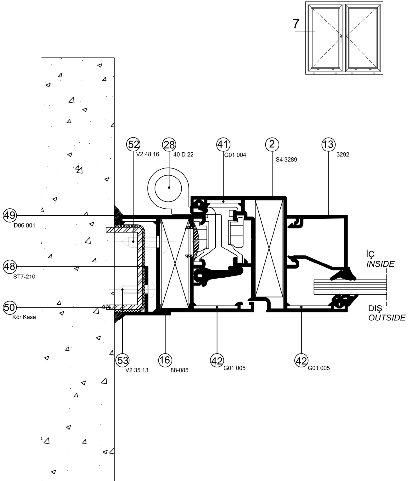
DETAIL 7 DETAYI
