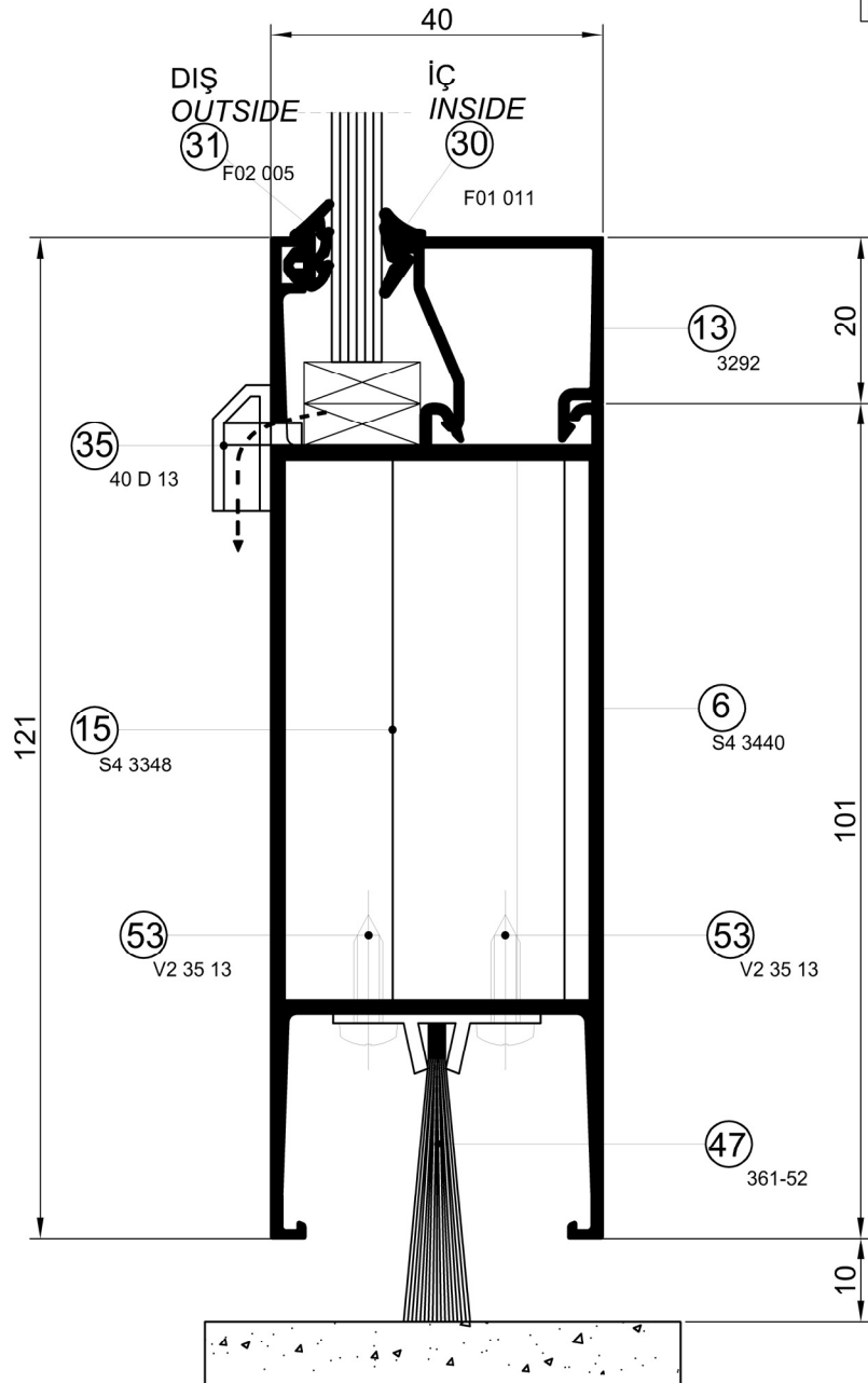
DETAIL ④ DETAYI
